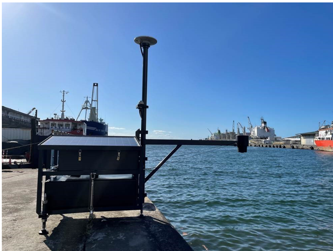
Figure 5 The Portagaugage deployed at Toamasina, Madagascar
